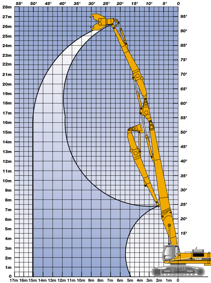
Demolition equipment
